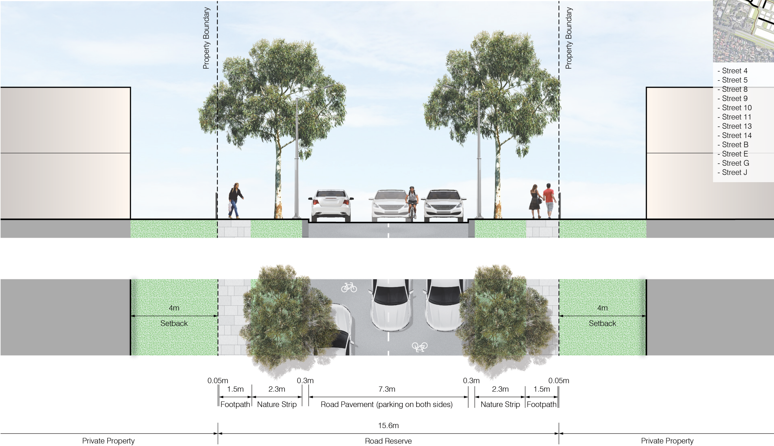
Figure 18: Typical Street 15.6m Profile
