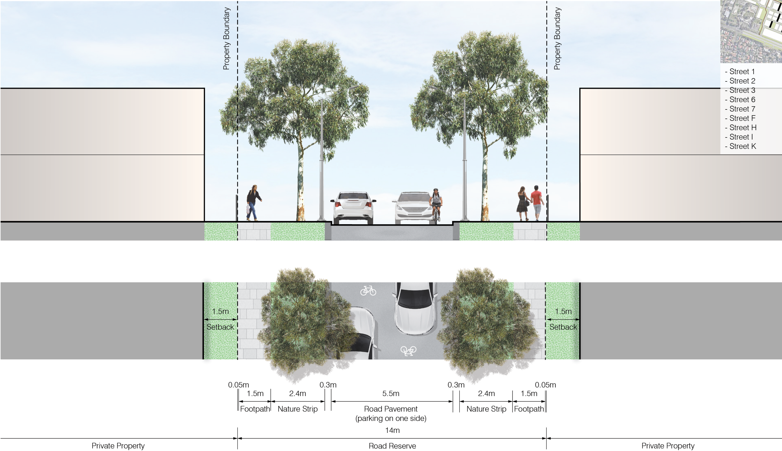
Figure 19: Typical Street 14m Profile
